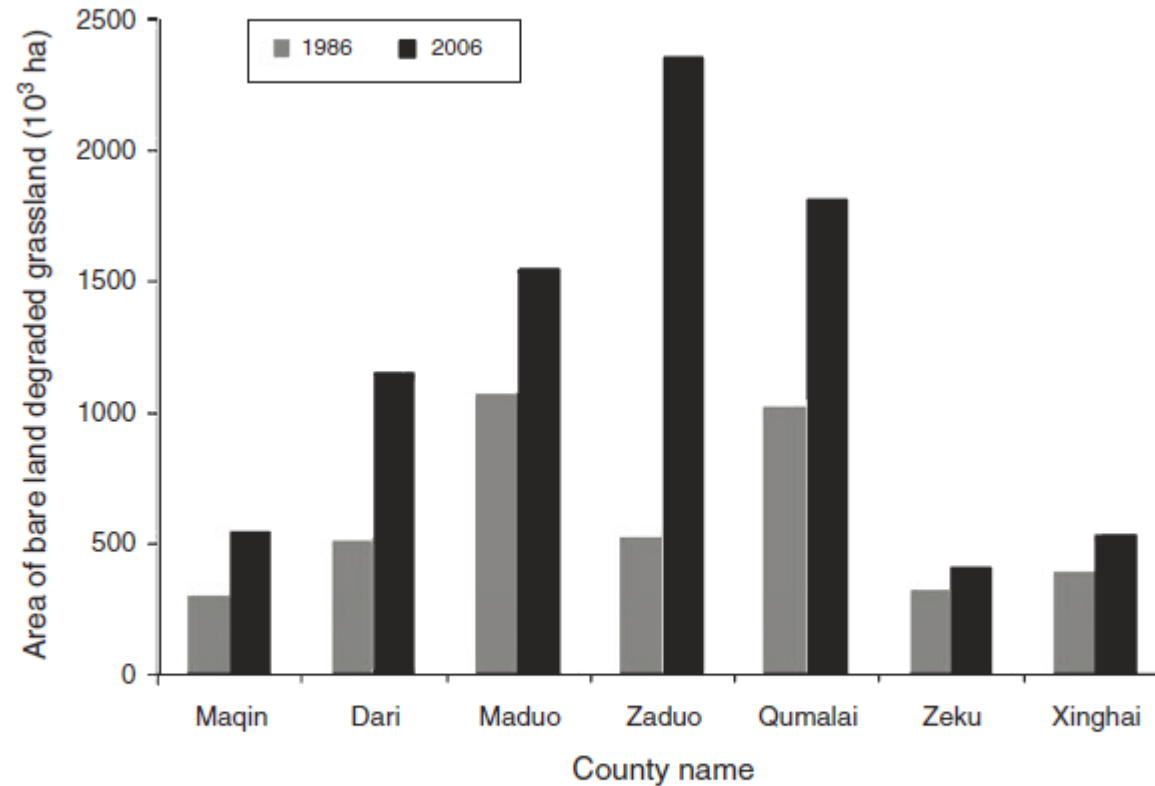
Fig. 3. Changes in the area of bare-land degraded grassland between 1986 and 2006 in seven counties within the Qinghai province (Maqin, Zeku, Xinghai, Dari, Zaduo, Qumalai and Maduo) in the headwater area of Yangtze and Yellow rivers (data from Ma 2007).
