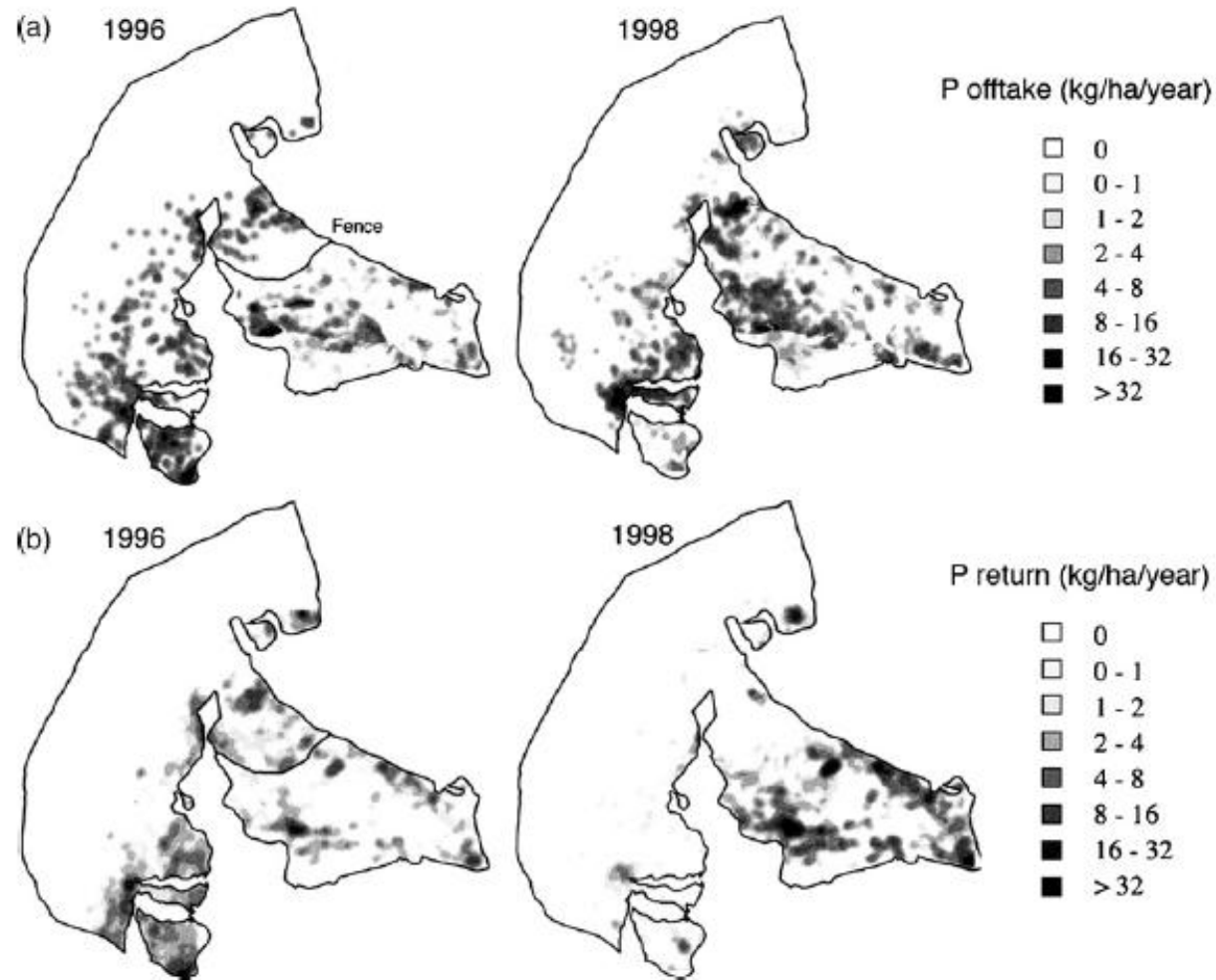
Fig. 2. Modelled distributions of (a) P offtake and (b) P return resulting from 100 days of cattle grazing on Alpe Nisciora.
