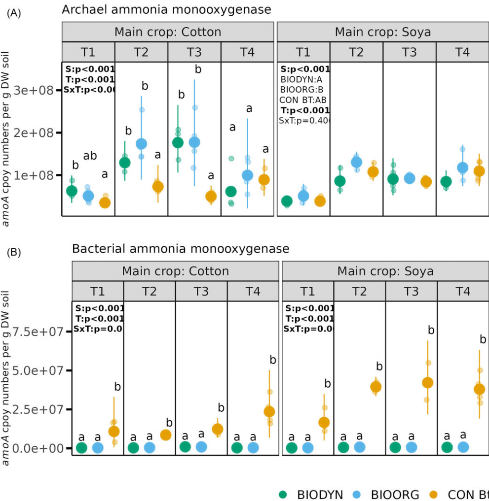
Figure 3. Treatment effects on bacterial and archaeal amoA abundance as assessed with quantitative real-time polymerase chain reaction (qPCR). Plots show raw data and estimated marginal means with 95% confidence intervals of linear mixed effect models assessing farming system (S) and crop cultivation phase (T) and the interaction effect (SxT) on bacterial and archaeal amoA abundance during cotton and soya cultivation phase. P-values of the main effects are presented within each plot in bold. Results of Sidak post hoc tests are indicated as small letters when a significant interaction effect was found. Without a significant interaction effect, Sidak posthoc tests were performed for systems across sampling dates, and results are given below the main effects in capital letters. BIODYN: biodynamic farming system; BIOORG: bio-organic farming system; CON Bt: conventional farming system with Bt cotton cultivation in the crop rotation.
