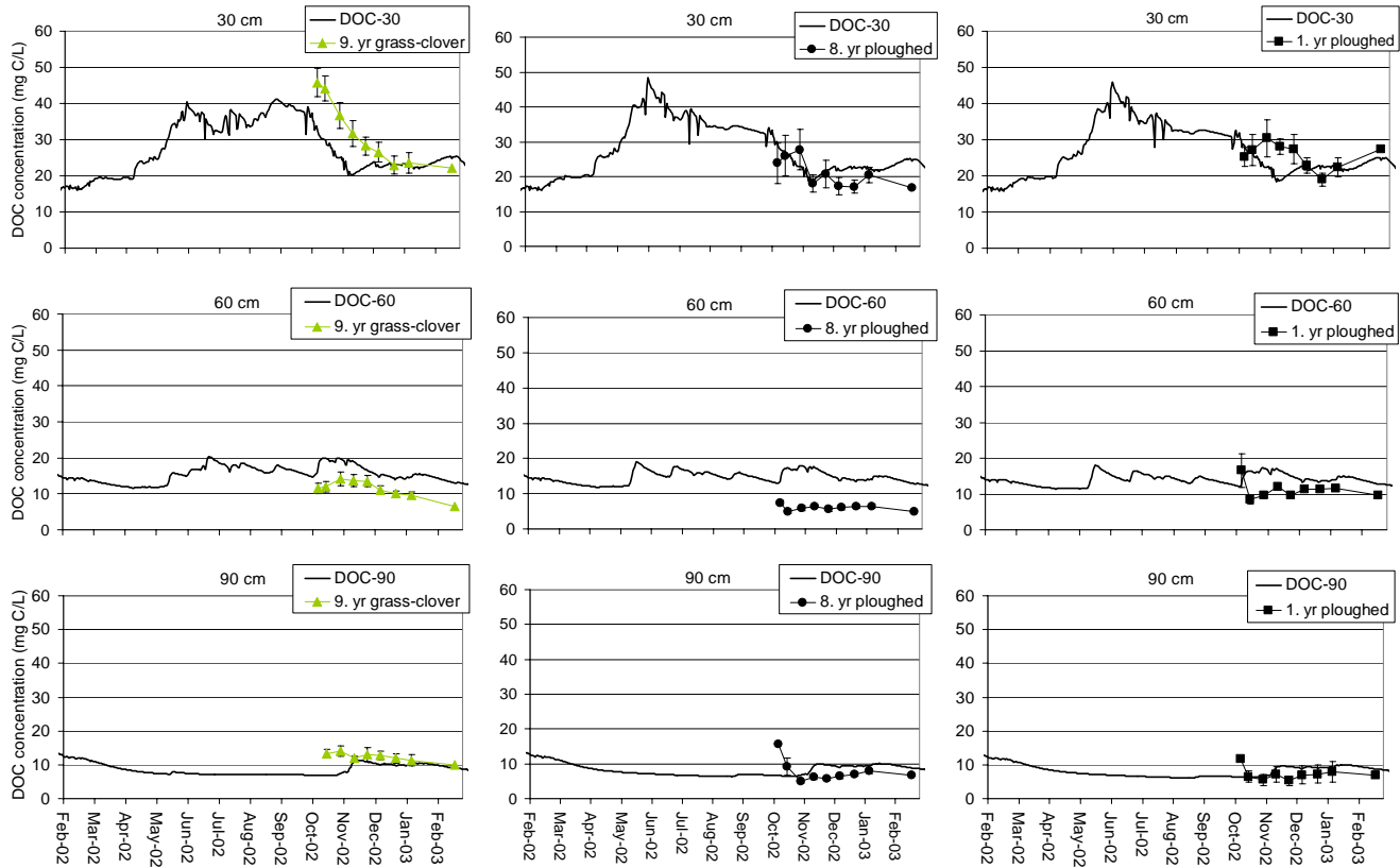
Figure 10. DOC concentration in suction cups (dots) (Vinther et al., 2005b) and simulated by the Daisy code (lines) in the Burrehøjvej field profiles at 30, 60, and 90 cm depth in three soil treatments: left figures: 9-year grass-clover with grazing cows. Middle figures: 8-year ploughed with grazing cows then soil ploughing. Right figures: 1-year ploughed with grazing cows then soil ploughing.
