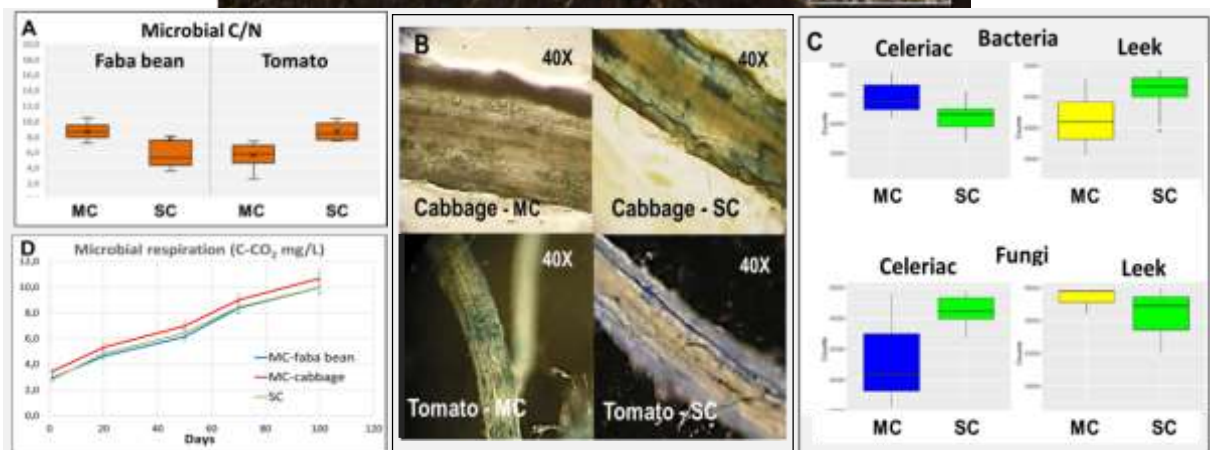
Figure 1: Overview of belowground biodiversity as affected by strip cropping in different SureVeg field trials. A: soil microbial C/N ratio in faba bean-tomato system (CREA-OF, Italy). B: Slightly- mycorrhized root of cabbage (Aarhus Univ., Denmark, 2019) and mycorrhized root of tomato (CREA, Italy) under strip cropping. C: Total counts of bacteria and fungi in celeriac-leek system by Next Generation Sequencing (ILVO-Inagro, Belgium). D: cumulative soil microbial respiration in faba bean-cabbage system (LatHort, Latvia).
