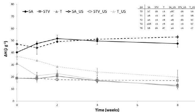
Fig. 5. Melting enthalpy ( \Delta H , J·g -1 ) of osmodehydrated cranberries with or without US pre-treatment during storage at 10 °C. Different letters indicate statistical differences ( p < 0.05 ) (lowercase letter within the same row indicate differences among different treatments for the same storage time, while capital letters within the same column indicate differences among different storage times for the same treatment).
