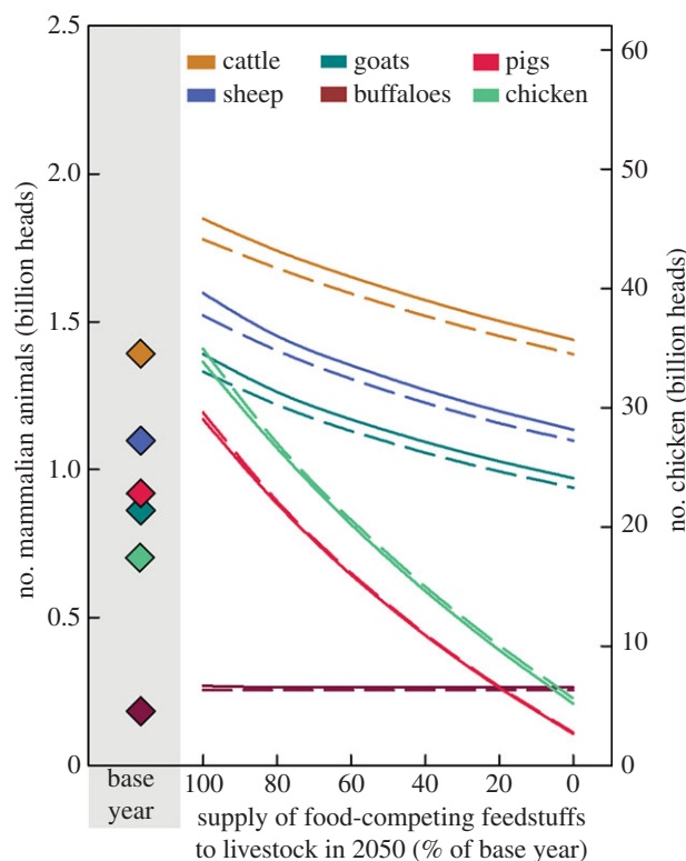
Figure 3. Livestock numbers in the base year, reference scenario, i.e. no reduction in food-competing feedstuffs (=100%) and with reduced usage of such feedstuffs. Diamonds (filled diamonds): levels in the base year. Solid lines: negative impact of climate change (CC) on yields absent; dashed lines: CC impact present.
