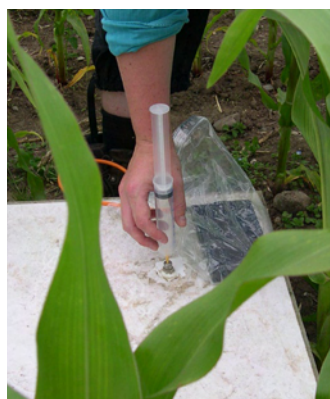
Figure 2. Emission of N 2 O was measured by manual gas sampling in gas-flux chambers.
