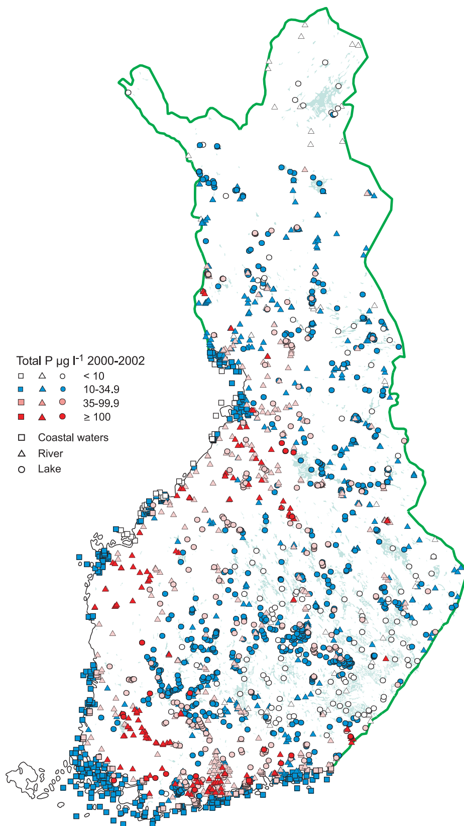
Figure 3. Average concentrations of total phosphorus ( \mu\text{g l}^{-1} ) in Finnish lakes, rivers and coastal waters in 2000–2002 based on summer data.
