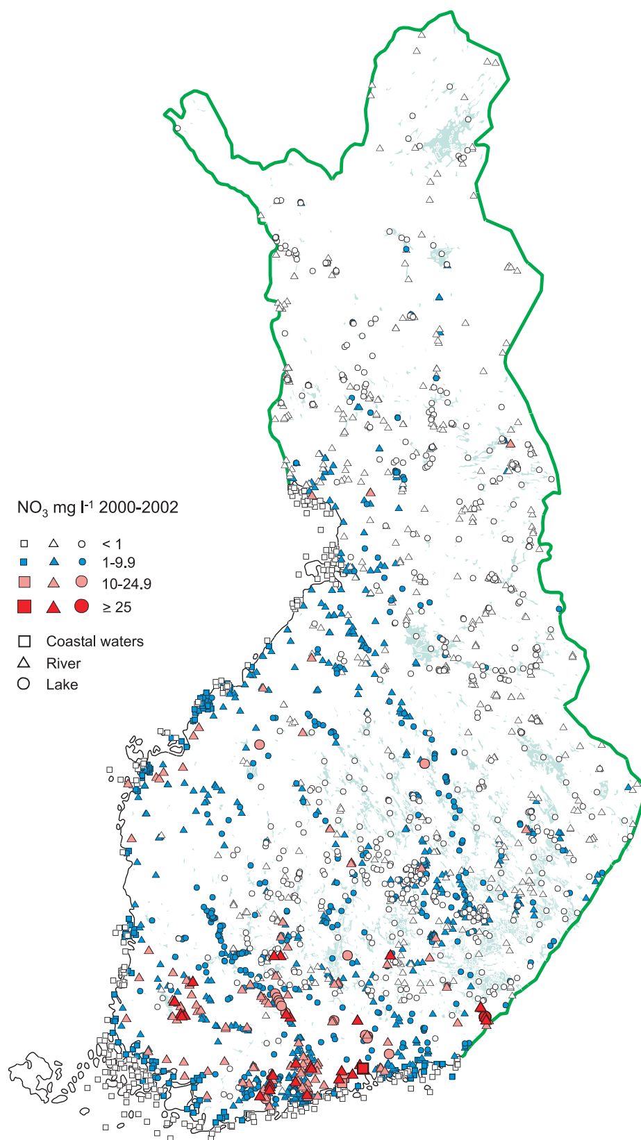
Figure 1. Maximum concentrations of nitrate (mg l -1 NO 3 ) in Finnish lakes, rivers and coastal waters in 2000–2002 based on data for the whole year.
