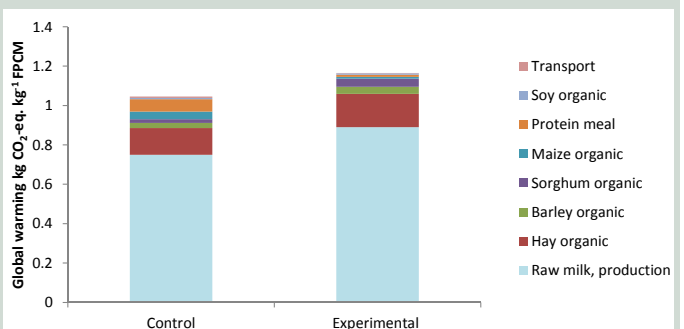
Figure 1 - Global warming potential of control and home-grown feed systems and the contribution from different processes
