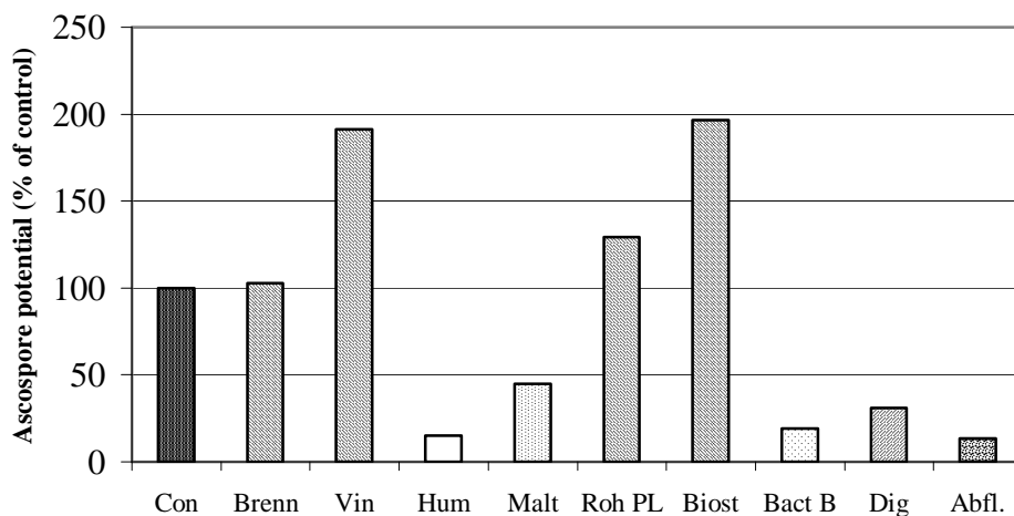
Figure 4: Leaf decomposition trial in Weinsberg 2002/2003. Cumulated ascospore potential in % of the control (black), cumulation of 13 dates up to May 23 rd .
